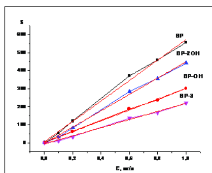
Fig.6. Calibration curves for benzophenones (after DME).
